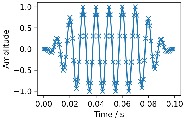
Signal downsampled to f_c=1\text{kHz}
