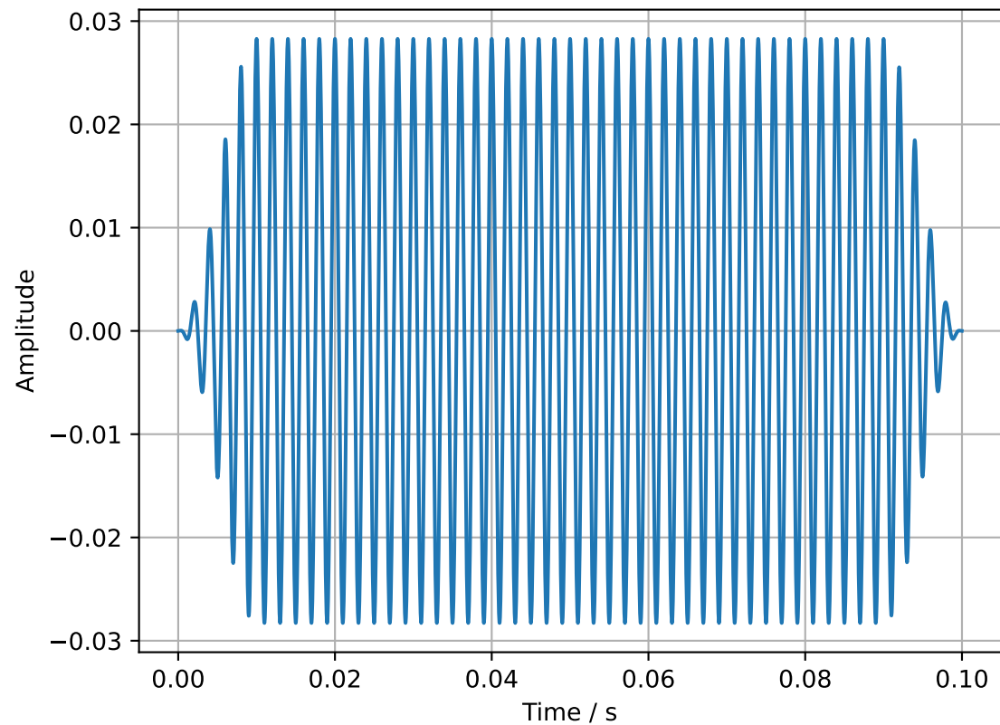
100ms 500Hz Tone with Raised Cosine Fades
