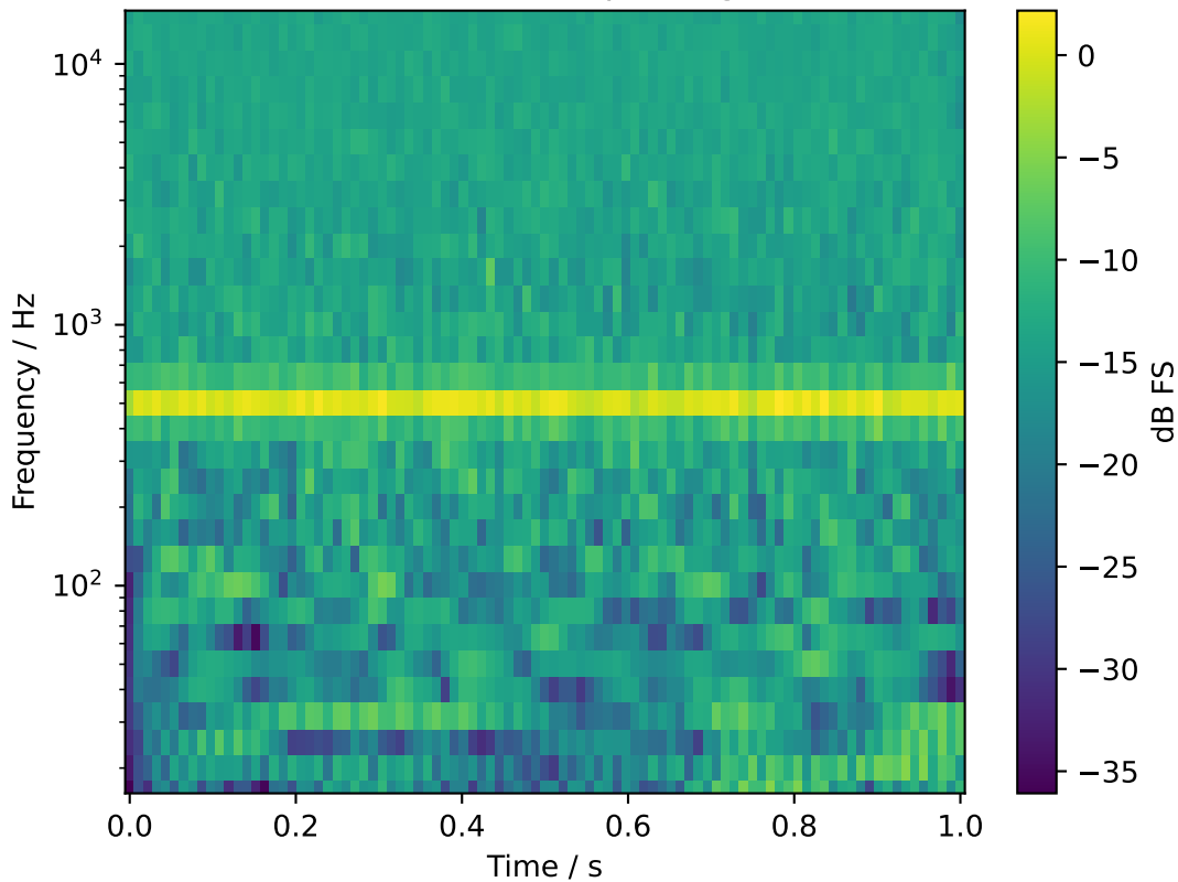
1/3 Octave-band spectrogram
