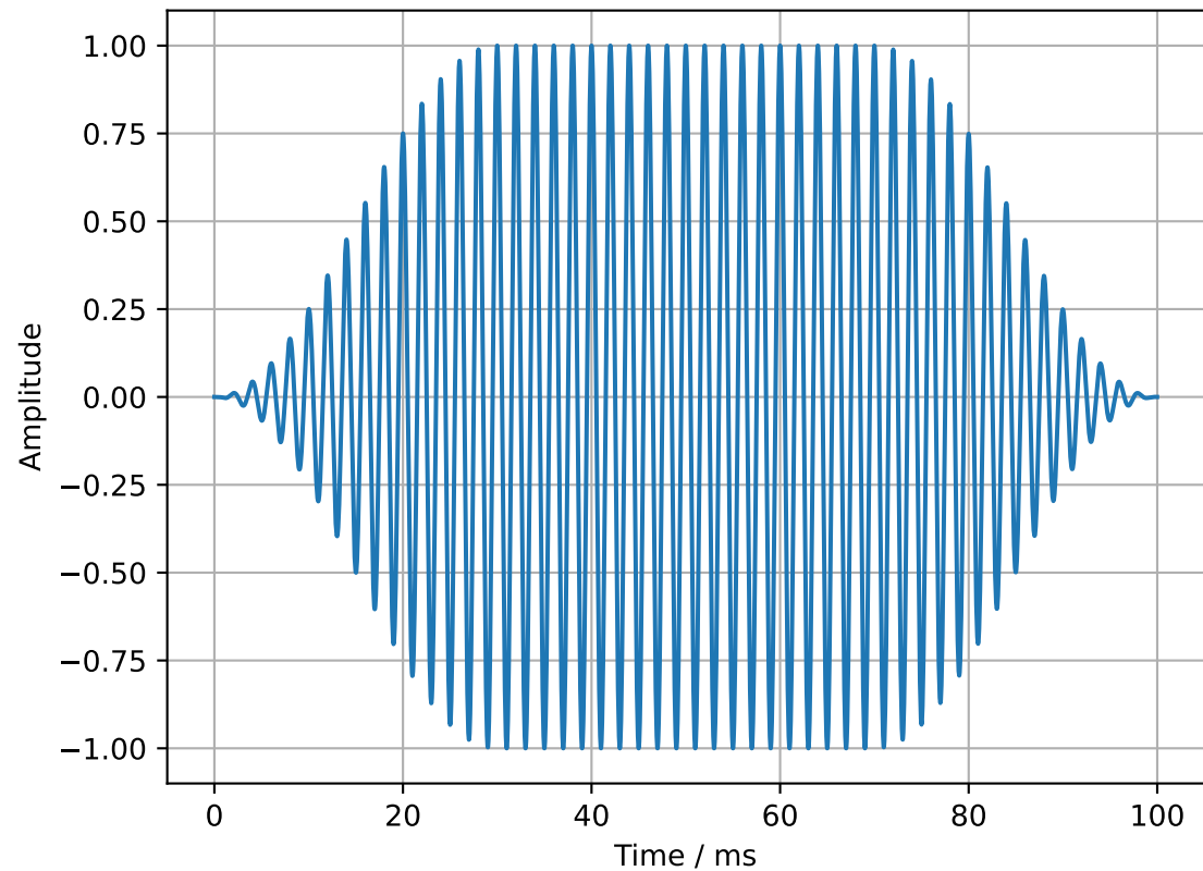
Tone with Raised Cosine Fade-in and -out
